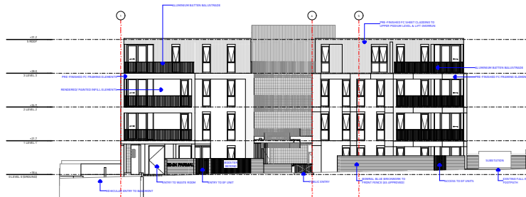
2 SOUTH (STREET) ELEVATION 1:500
