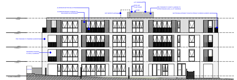
4 EAST ELEVATION 1:500
