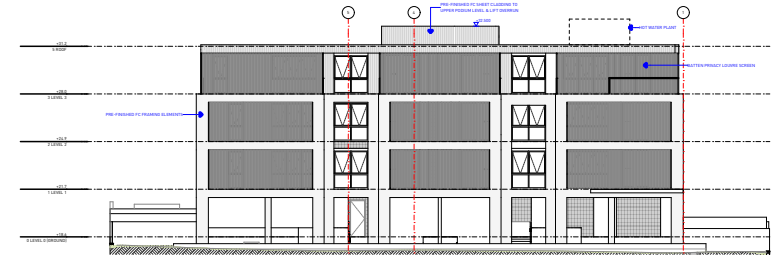
3 NORTH (REAR) ELEVATION 1:500
