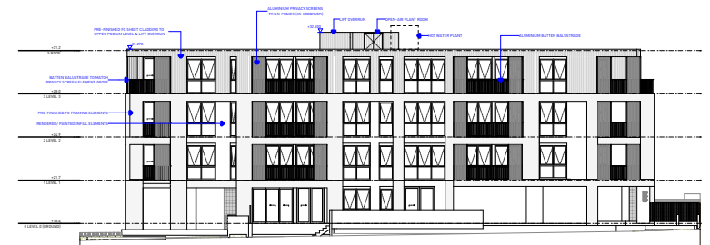
5 WEST ELEVATION 1:500
